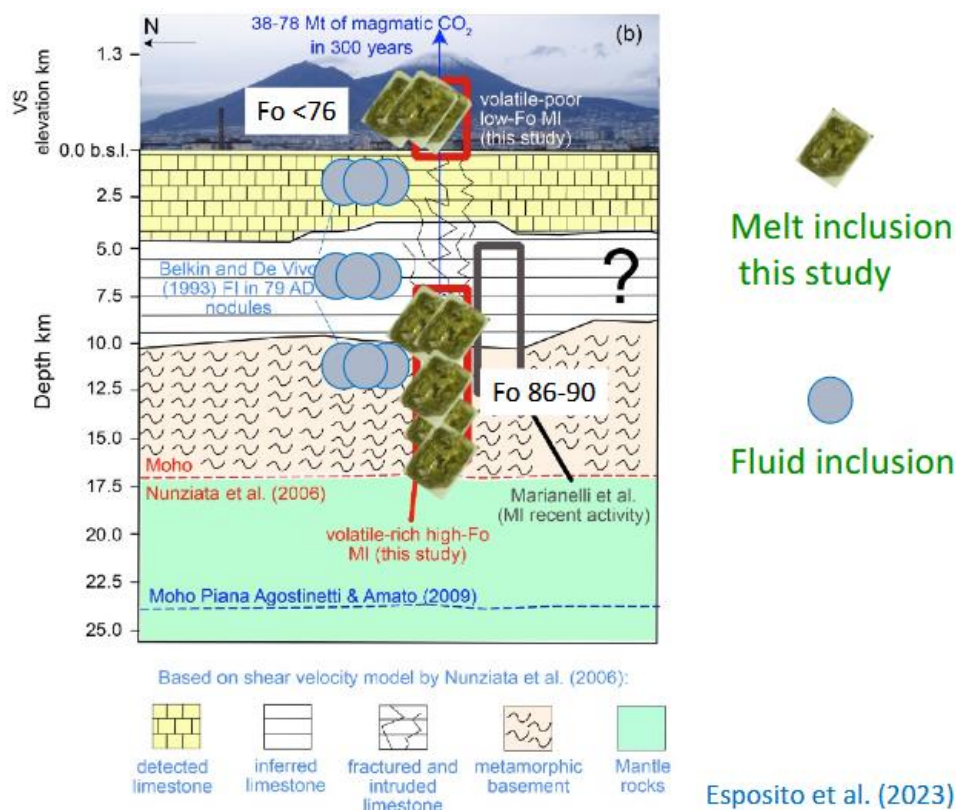
Geological schematic cross section of Mount Somma-Vesuvius (modified from Esposito et al. (2023)).
