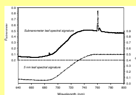
Comparison of a subnanometer leaf spectral signature derived from the HR2000 devices and a reference green leaf reflectance recorded by a traditional spectrometer with spectral resolution of 5 nm.
