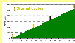
Ozone AOT40 over the course of the experiment and days of measurement.
